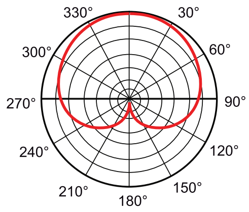
Cardioid Polar Pattern
